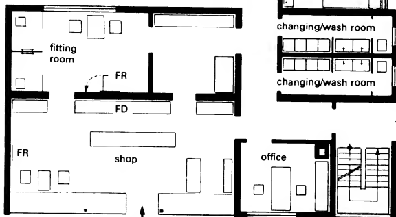
② Example of a tailor's (ground floor)
